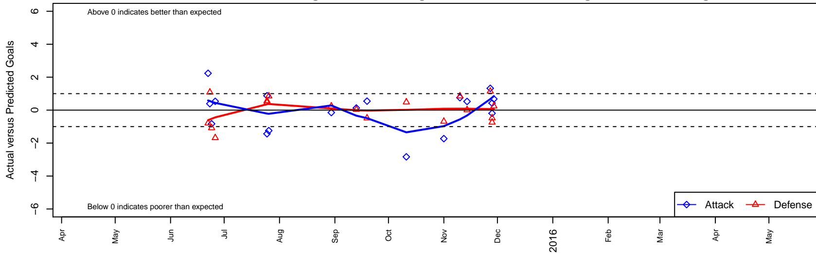
Santa Clara Sporting Green G99 Dots are actual minus expected GF (blue circles) and GA (red triangles). Blue line is smoothed change in attack strength. Red is smoothed change in defense strength.
